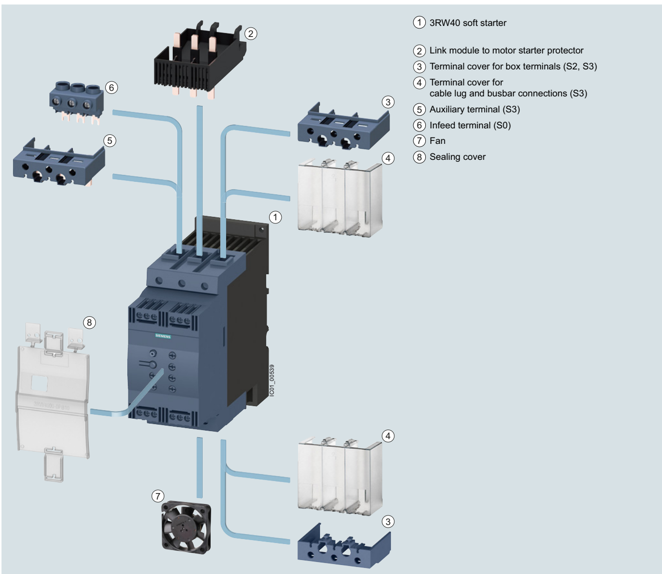
3RW40 Basic Performance soft starters with accessories (see page 6/94)
