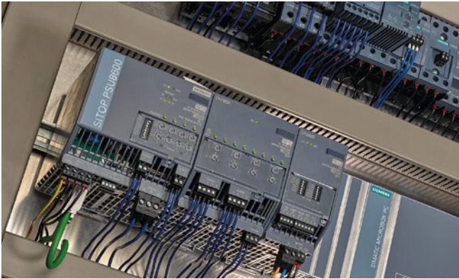
SITOP PSU8600 – a new 4 x 5 A basic unit enables the unique functions of the power supply system to be used in 1-phase systems – see page 6/7.
